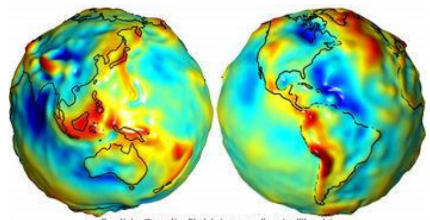
Earth's Gravity Field Anomalies [milligals] -50 -40 -30 -20 -10 0 10 20 30 40 50
